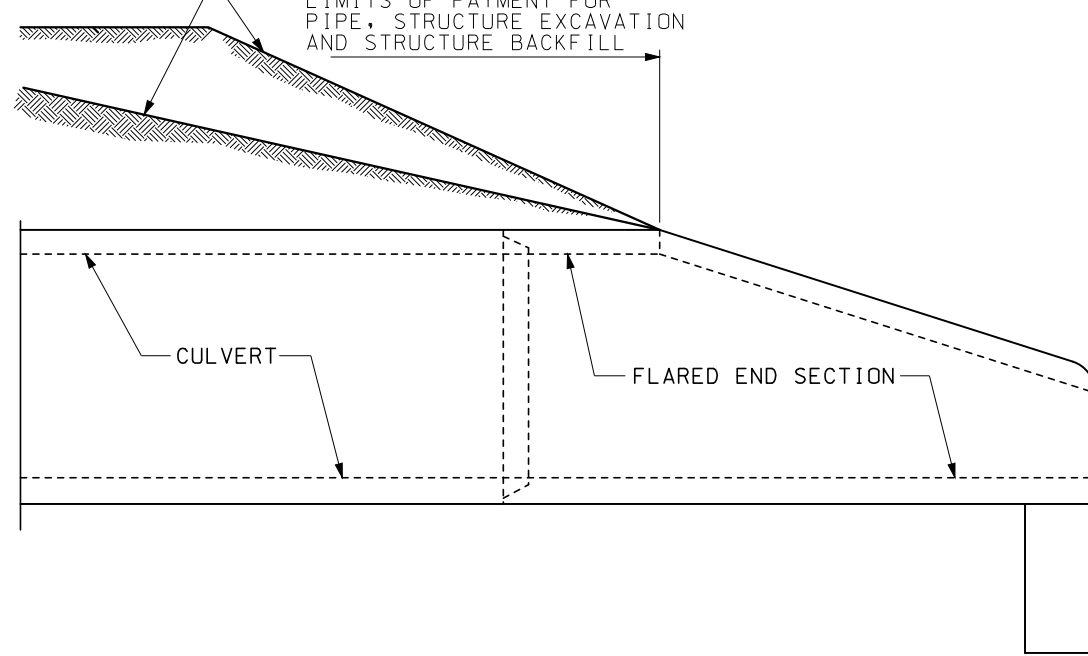
INSTALLATION DETAILS
